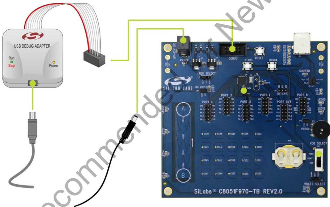
Figure 2. Hardware Setup
